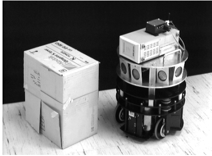
(a) OBELIX robot
