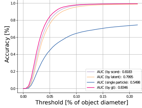
Figure 2. Accuracy Curve with AUC values for all selection methods for a model trained and tested on all objects. Single particle sampling, i.e. eliminating the need for any selection strategy yields the lower bound and selection by ground truth information the upper bound.
