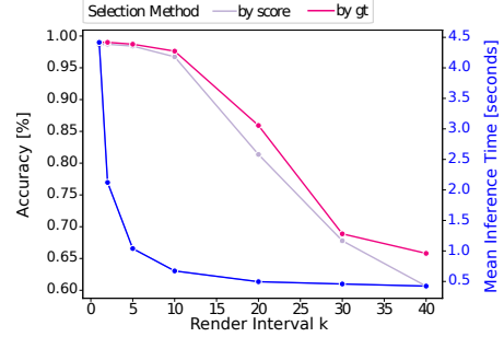
Figure 3. Relation between the rendering interval k , accuracy, and inference runtime. The interval k controls how often the point cloud is rendered and encoded during inference; in other iterations, only the latent vector z_o is transformed. Results are based on 100 iterations, 20 sampled particles, and the driller object.
