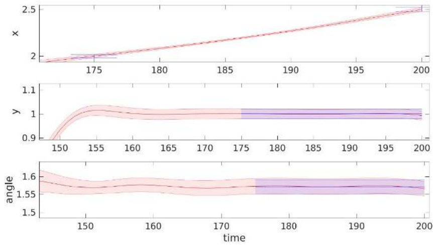
Figure 2.7.: The achieved distribution (red) was estimated based on 1000 samples and compared to the target distribution (blue) in the vicinity of specified time steps. Our approach accurately matches mean and variance for all three task variables. ©2016 IEEE.
