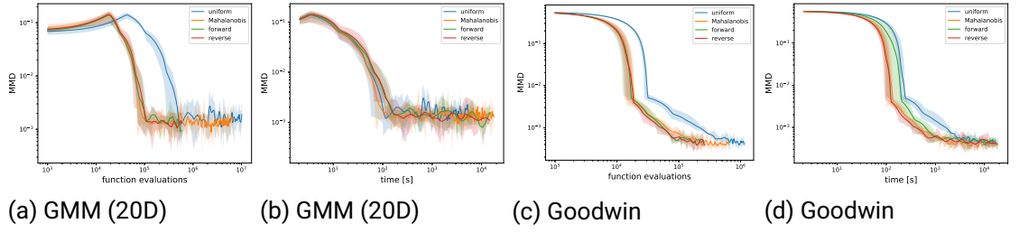
Figure B.1.: Using the Mahalanobis distance as dissimilarity measure results in similar sample efficiency compared to using the KL divergence while adding less computational overhead.
