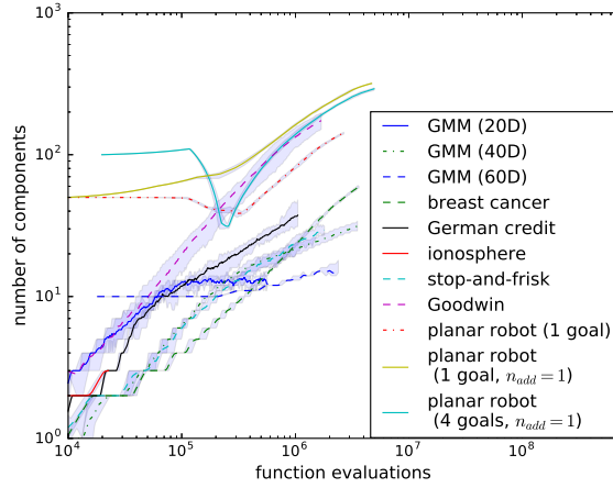
Figure B.5.: The average number of components learned by VIPS++ is plotted over function evaluations for all experiments in the test bed. When using the faster adding rate, n_{\text{add}} = 1 , VIPS++ learns GMMs with approximately 350 components.
