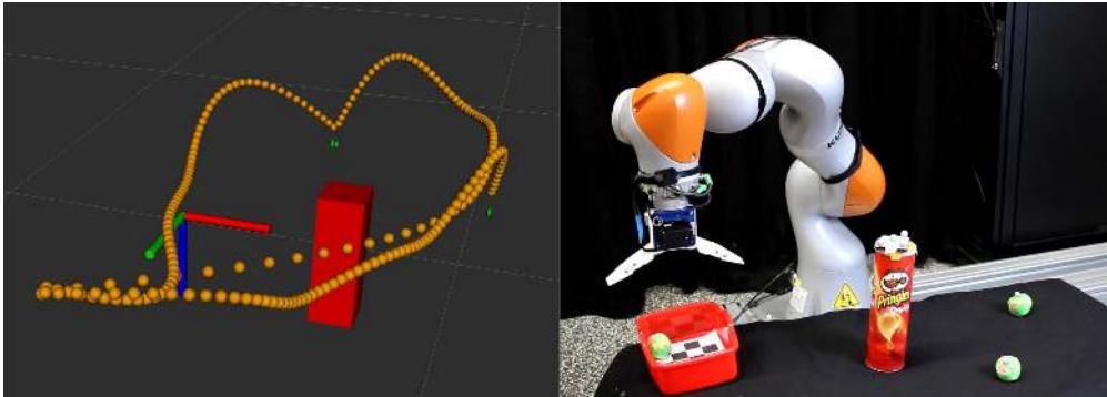
Figure 3.12.: We performed experiments on a Kuka IIWA R820 robot where we re-planned the mixture of ProMPs online. Re-planning was triggered when new obstacles appeared or when objects where grasped or released. The left image shows the visualization of the learned plans that was shown to the operator. For better visualization, the (variable) stiffness was not visualized. Image was taken from [Ewerton et al., 2020].
