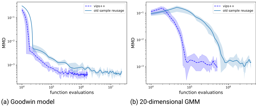
Figure 3.5.: The sample reuseage of VIPS++ is approximately one order of magnitude more efficient than the sample reuseage of VIPS.
